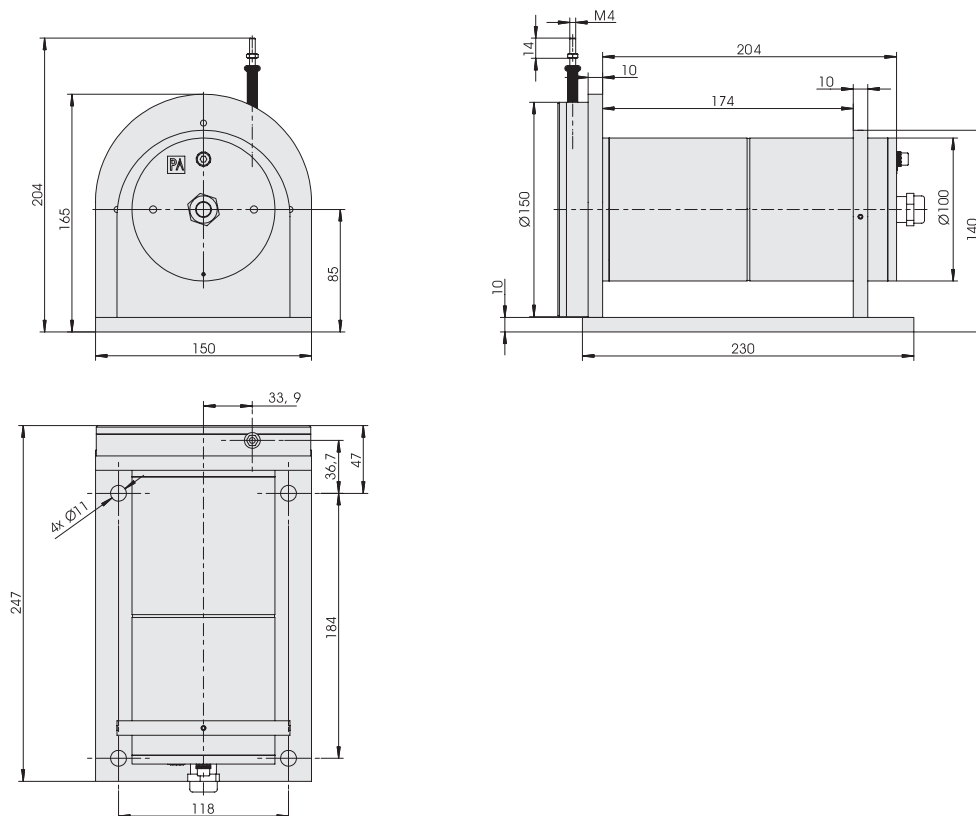
Outline drawing WS100 - 2000
